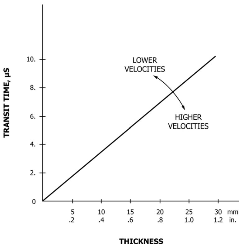
FIG. 1 Transit Time/Thickness Relationship
